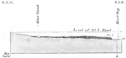
Section of Glen Turret detrital terrace mound from the Turret at the foot of the pass into Glen Gluoy to the River Roy, a distance of 1 mile.
